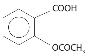
acetylsalicylic acid
