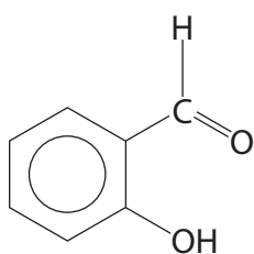
salicylaldehyde
