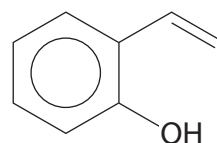
compound F
