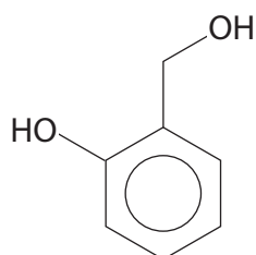
salicyl alcohol
