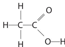
ethanoic acid
